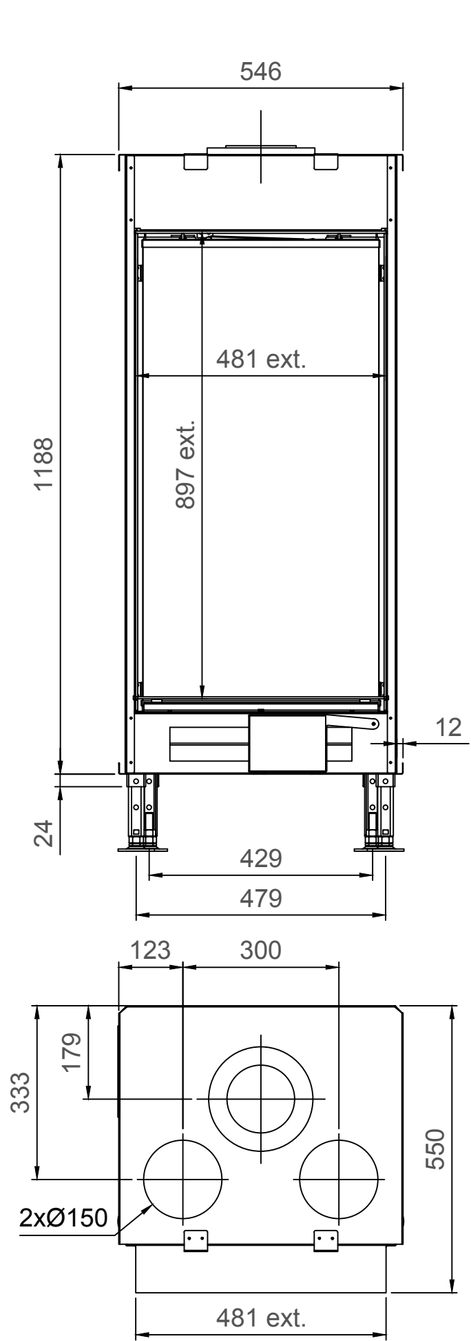
True Vision 550V - Type 4 - 90mm
