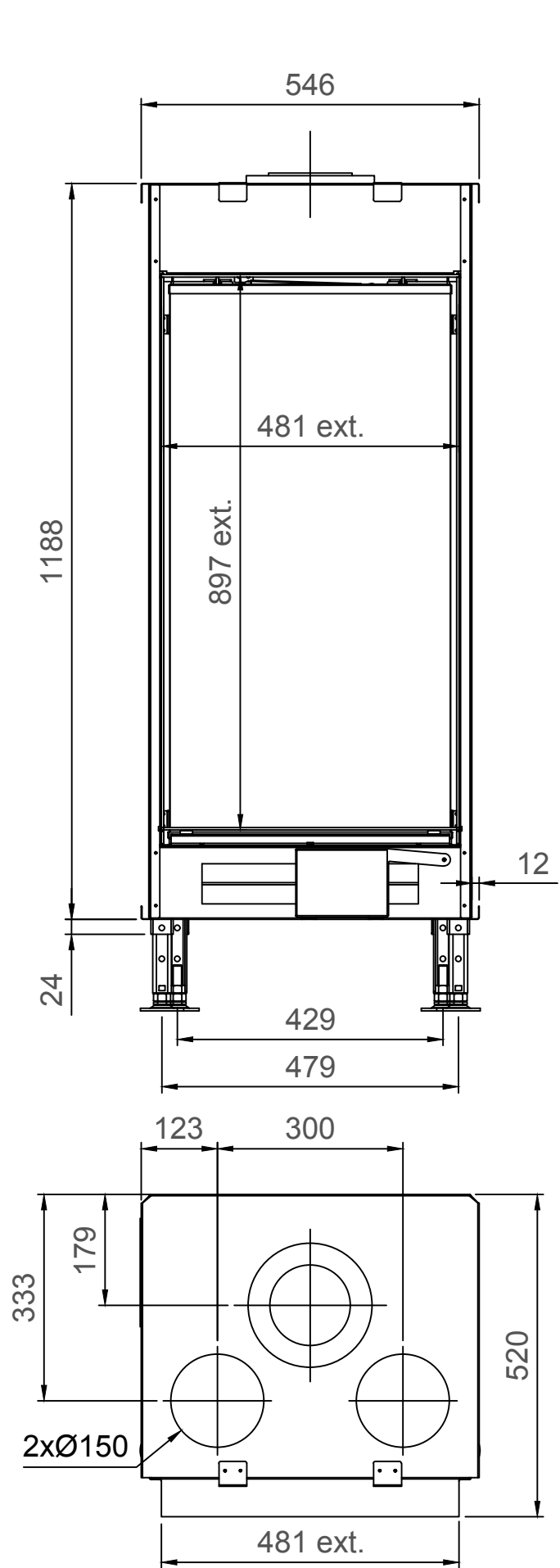
True Vision 550V - Type 4 - 60mm
