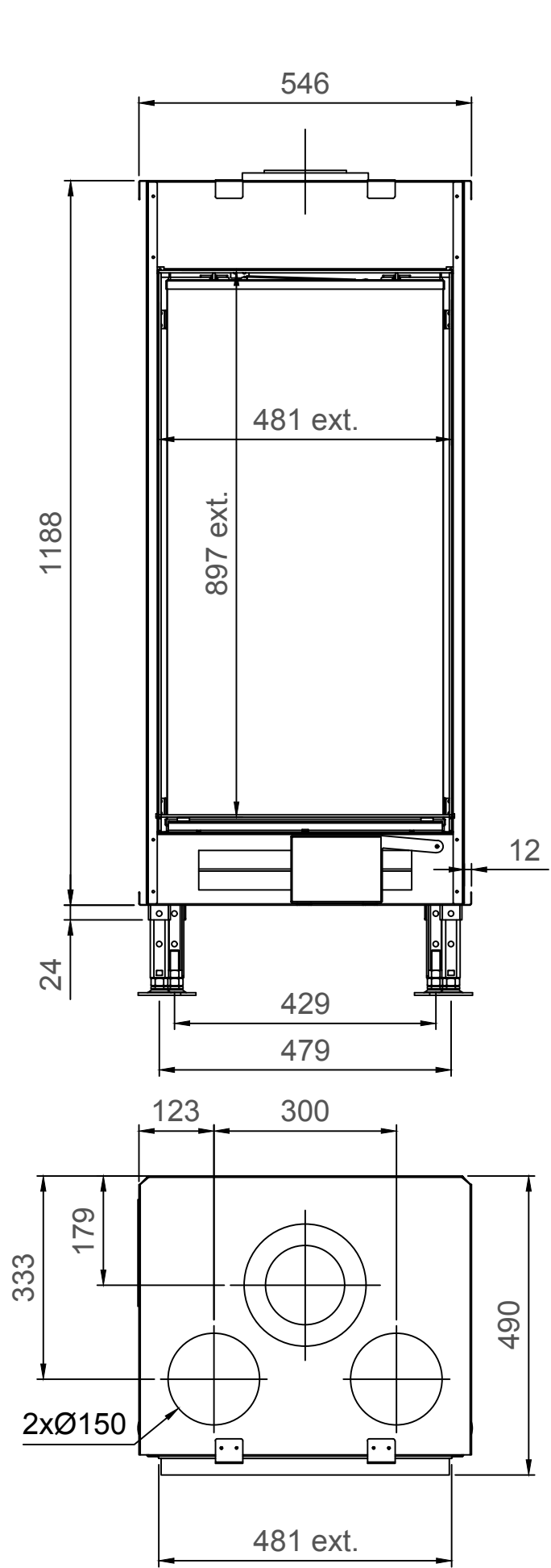
True Vision 550V - Type 4 - 30mm
