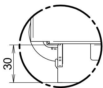
DETAIL A 1:2
