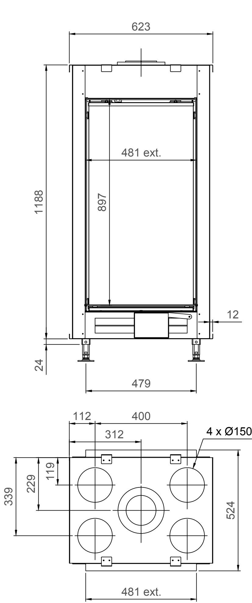
True Vision 550DV - Type 4 - 30mm
