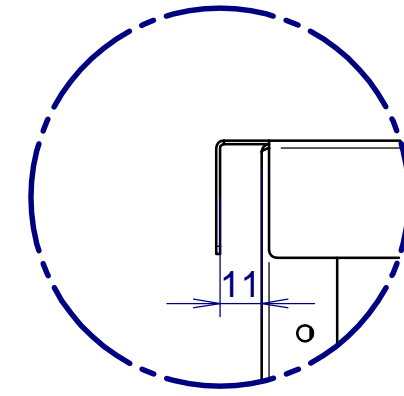
DETAIL A 1:2
